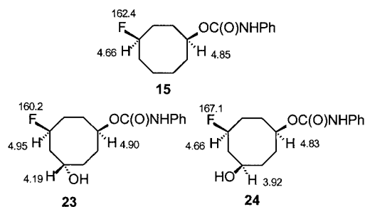
Scheme 7. Characteristic ^1\text{H} and ^{19}\text{F} NMR chemical shifts of compounds 15 , 23 , and 24
