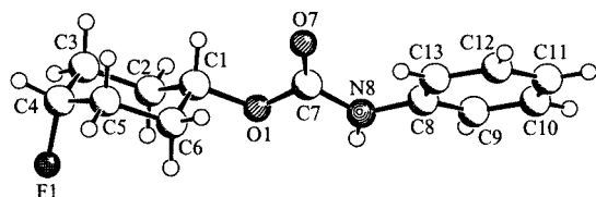
Figure 1. Crystal structure of compound 9
