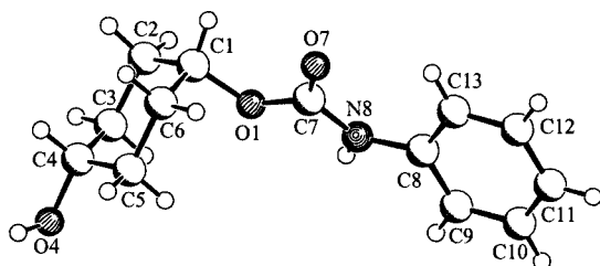
Figure 4. X-ray crystal structure of compound 17
