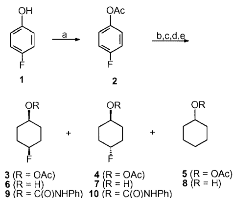
Scheme 1. Reagents and conditions: (a) \text{Ac}_2\text{O}/\text{Py} , 3 h, reflux; (b) \text{RhCl}_3/\text{Aliquat 336}/1,2\text{-dichloroethane}/\text{water} ; (c) \text{KOH}/\text{MeOH} , 2 h, room temp.; (d) chromatography; (e) \text{PhCNO} , petroleum ether 110–140 °C, reflux, 4 h
