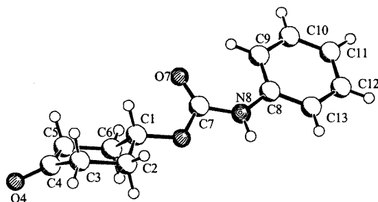
Figure 3. X-ray crystal structure of compound 16
