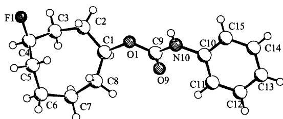
Figure 2. Crystal structure of compound 15
